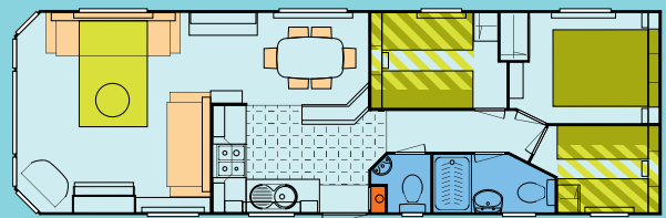
37/3 Bedroom 8 Berth Body Length (inc. bay) - 11.59m (38'-0 3/4") Body Width - 3.69m (12'-1")
