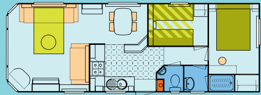
32/2 Bedroom 6 Berth Body Length (inc. bay) - 10.33m (33'-10 3/4") Body Width - 3.69m (12'-1")
