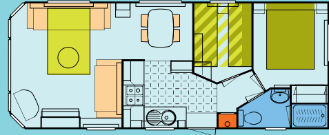
28/2 Bedroom 6 Berth Body Length (inc. bay) - 9.21m (30'-2 3/4") Body Width - 3.69m (12'-1")
