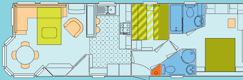
39/2 Bedroom Body Length (inc. bay) - 12.32m (40'-5 1/4") Body Width - 3.79m (12'-5")
