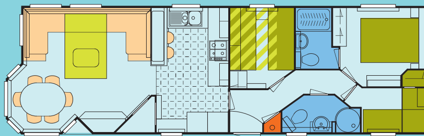
39/3 Bedroom Body Length (inc. bay) - 12.32m (40'-5 1/4") Body Width - 3.79m (12'-5")
