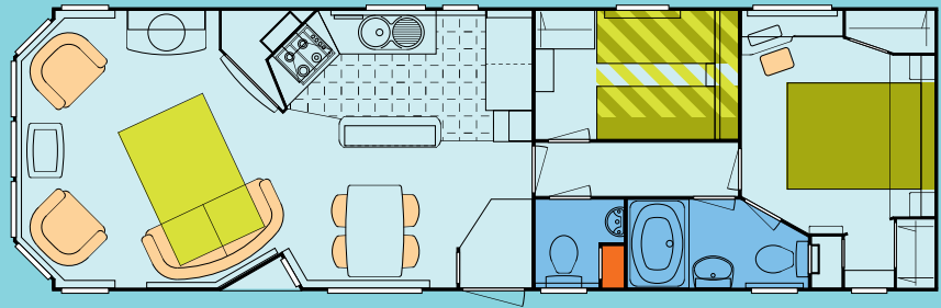
38/2 Bedroom Body Length (inc. bay) - 11.95m (39'-2 1/2") Body Width - 3.69m (12'-1")
