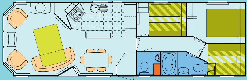
38/3 Bedroom Body Length (inc. bay) - 11.95m (39'-2 1/2") Body Width - 3.69m (12'-1")
